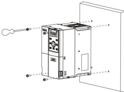
图 3-2 LS300T0.7GB/1.5PB ~ LS300T18.5GB/22PB, LS300-2T0.7GB/1.5PB ~ LS300-2T7.5GB/11PB
