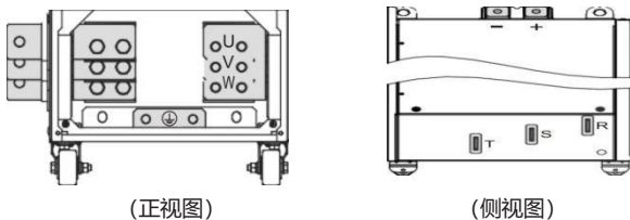
图 3-12 LS300T200G/220P-C ~ LS300T630G/710P-C主回路端子分布图
