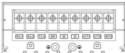
图 3-9 LS300T0.7GB/1.5PB ~ LS300T18.5GB/22PB, LS300-2T0.7GB/1.5PB ~ LS300-2T7.5GB/11PB主回路端子分布图
