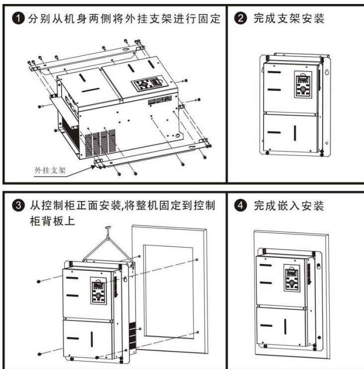
图 3-5 LS300T22GB/30PB~LS300T160G/200PB, LS300-2T11GB/15PB~ LS300-2T55G/75PB 机型嵌入式安装示意图
